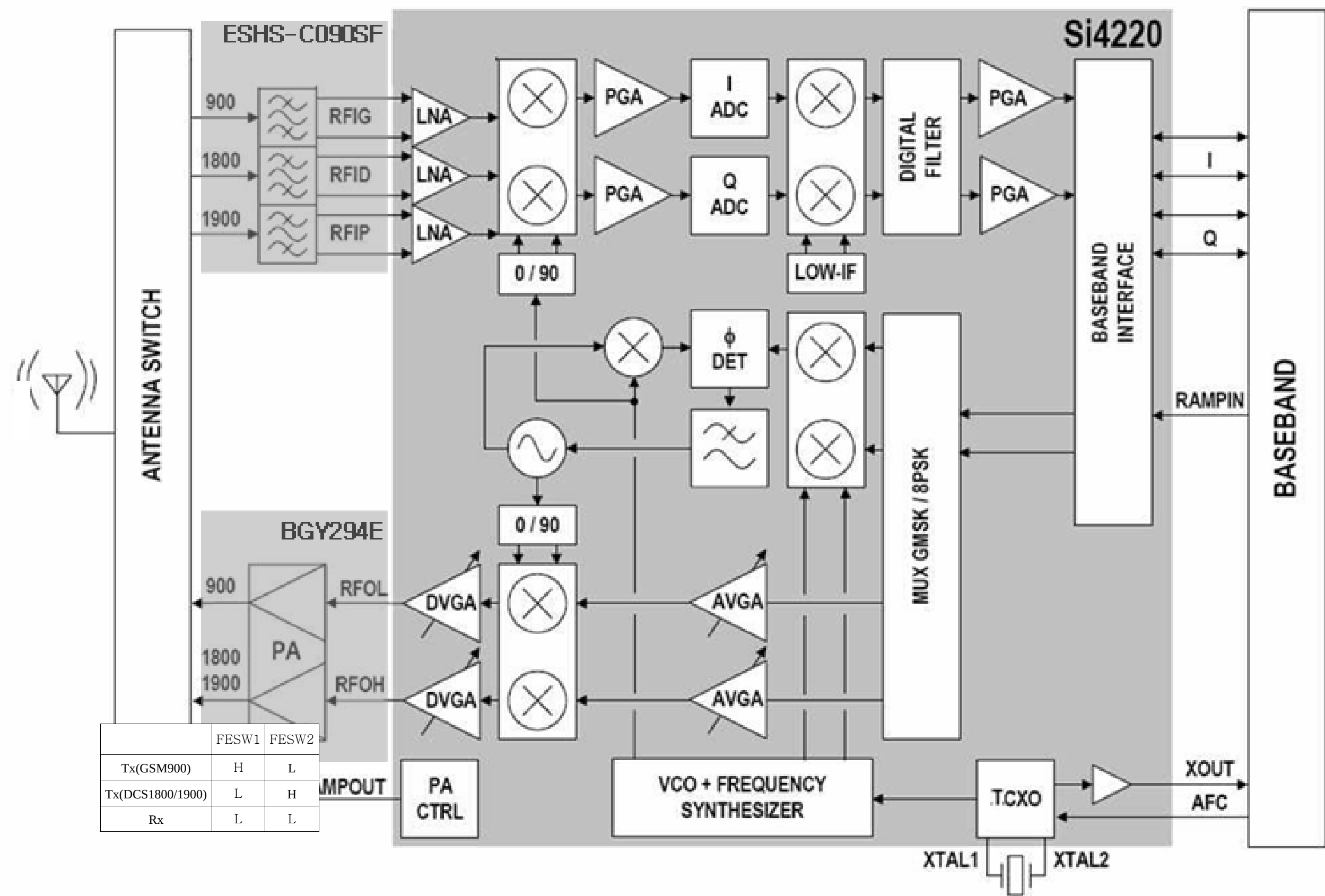
7-1. RF Solution Block Diagram
